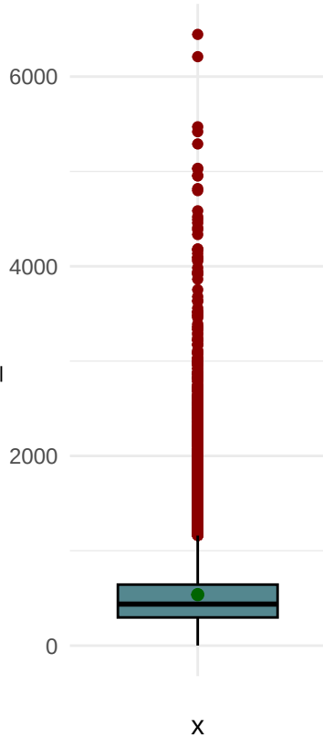
total_bedrooms
