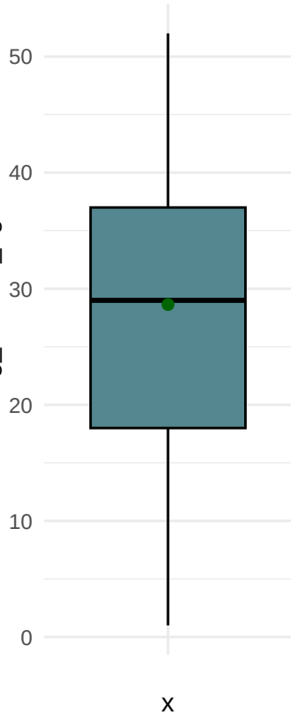
housing_median_age
